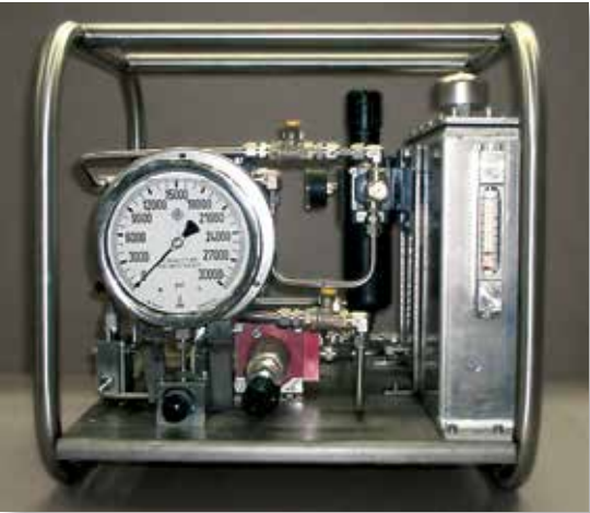
Power Unit for Stud Tensioner
